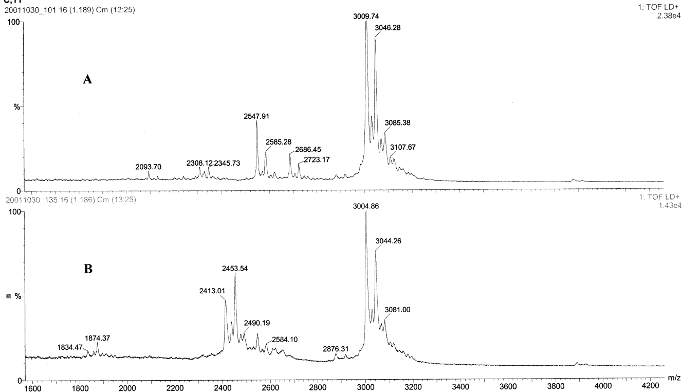
Figure 3. Typical spectra of S. aureus methicillin-susceptible strain (A) and methicillin-resistant strain (B).
